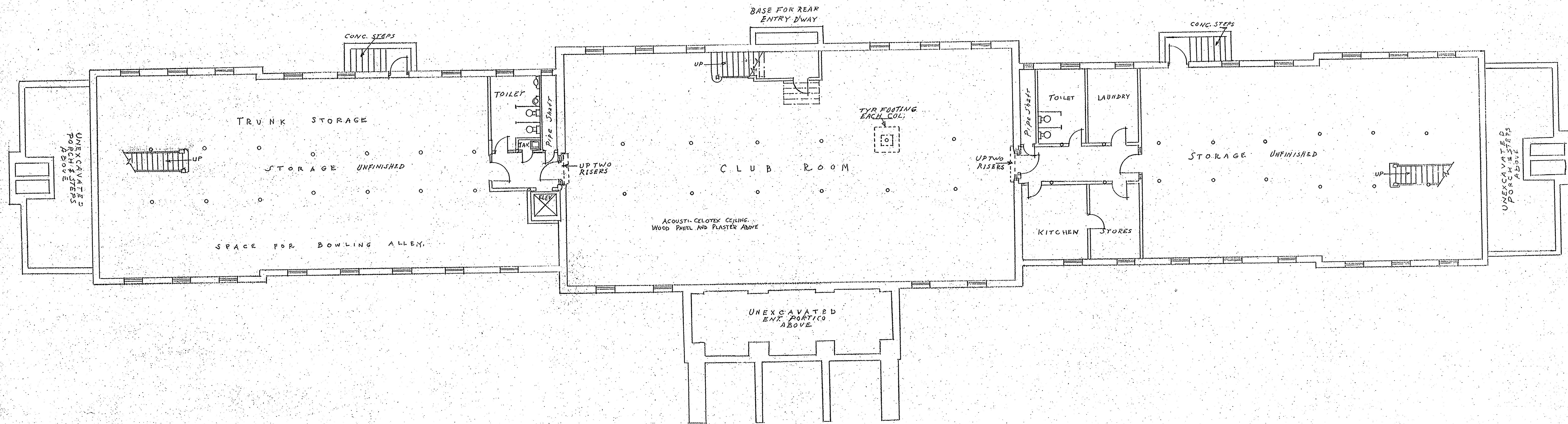
BASEMENT PLAN Scale 1/8" = 1'-0"
